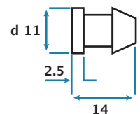
Remache de Silicona PSP001 (escala 3:1)
